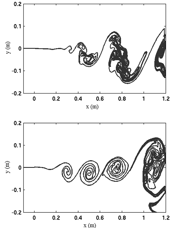
Fig. 11 Single realization of a shear-layer loci simulated using the weakly compressible model: a) unforced, and b) forced at 650 Hz with an amplitude of 2.5 mm.
