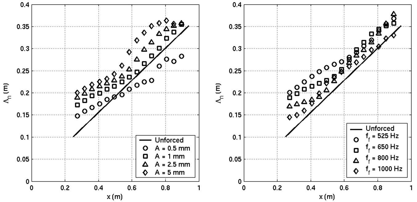
Fig. 10 WCM predictions of optical coherence length versus downstream distance for a forced shear layer with an upper stream velocity of u_U = 261.04 m/s and a lower stream velocity of u_L = 34.7 m/s: a) results for a shear layer with f_f = 650 Hz with varying forcing amplitudes, and b) results for a shear layer forced at varying frequencies with A = 2.5 mm.
